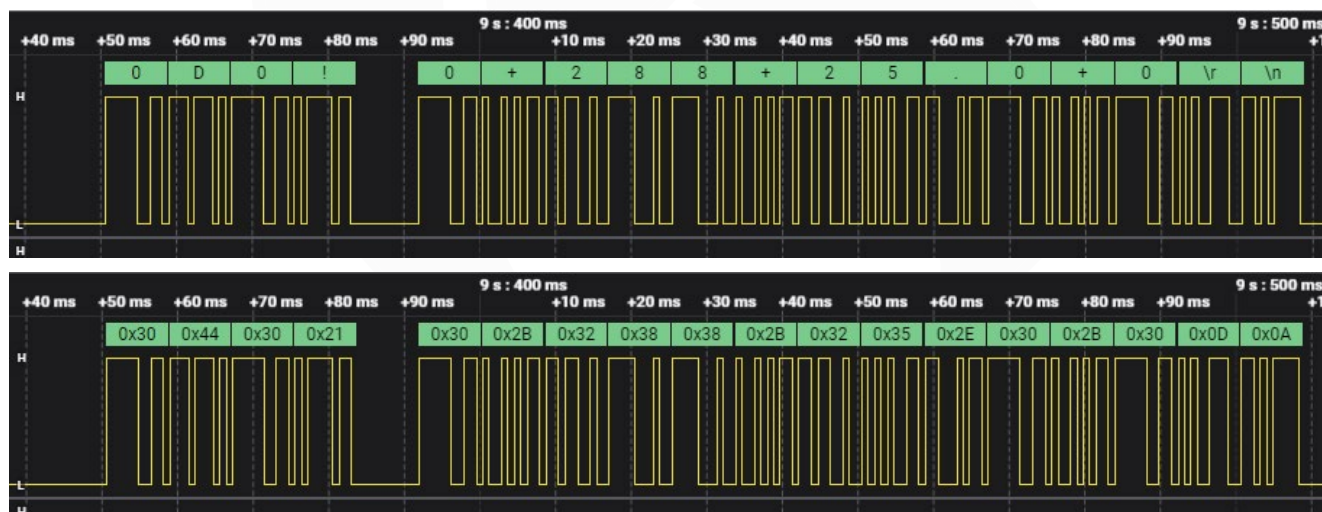
Figure 14. Oscillogram
