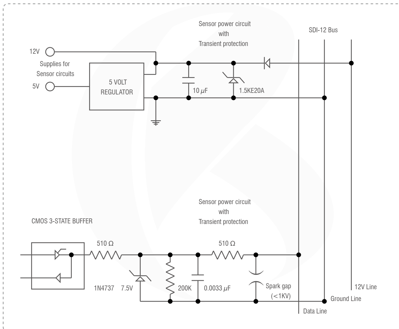
Figure 15. Recommended SDI-12 circuit
