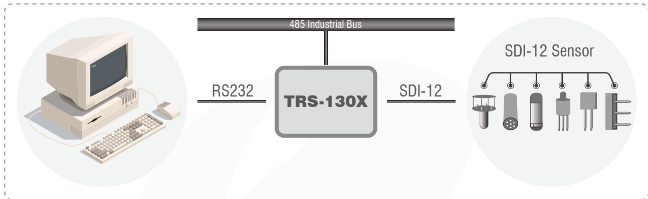
Figure 3. Diagram of converter hardware connection
